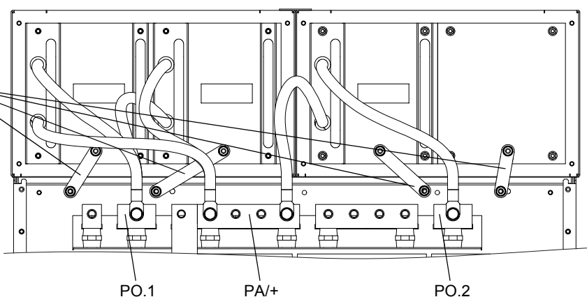
Example 3: ATV61HC40N4
